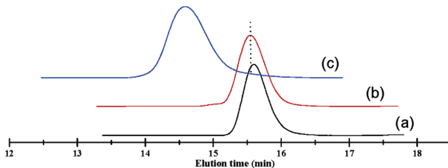
Figure 2. SEC traces for (a) PEO-RAFT, 2 ( M_n = 5400 amu; PDI = 1.04); (b) PS- b -PEO diblock, 3 ( M_n = 6900 amu; PDI = 1.06); and (c) PS- b -PMMA- b -PEO triblock copolymer, 4a ( M_n = 20\,800 amu; PDI = 1.05).
